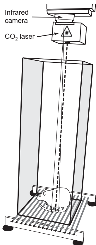
Fig. 1. The experimental setup used for testing the tail-flick. The dotted line shows the path of the CO 2 laser beam aimed at the midsection of the tail. The infrared camera, which was mounted next to the laser unit, was focused on the same area. The tail was brought under the laser beam by gently sliding the whole cage on the smooth surface of the bench.
